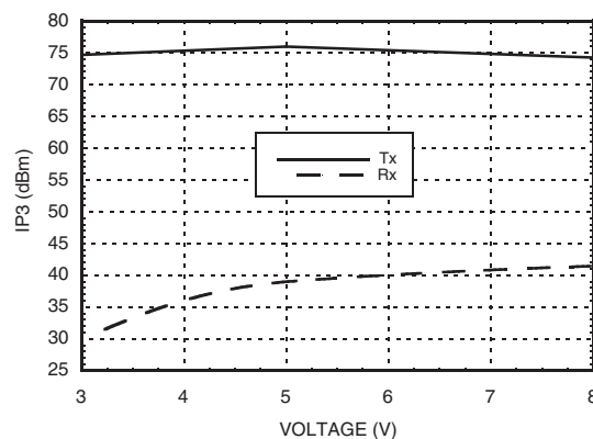
Input IP3 vs. Voltage with 1600 MHz Tuning
